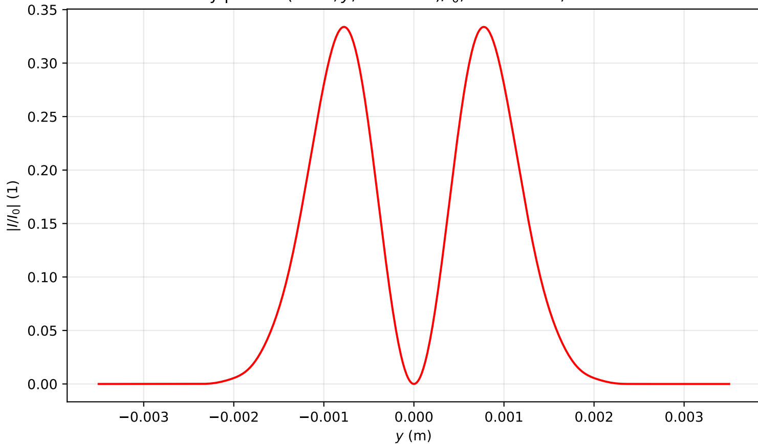
Intensity profile I(x=0, y, z=2.548)/I_0 , P_{in}=1.0P_{cr} , artificial time
